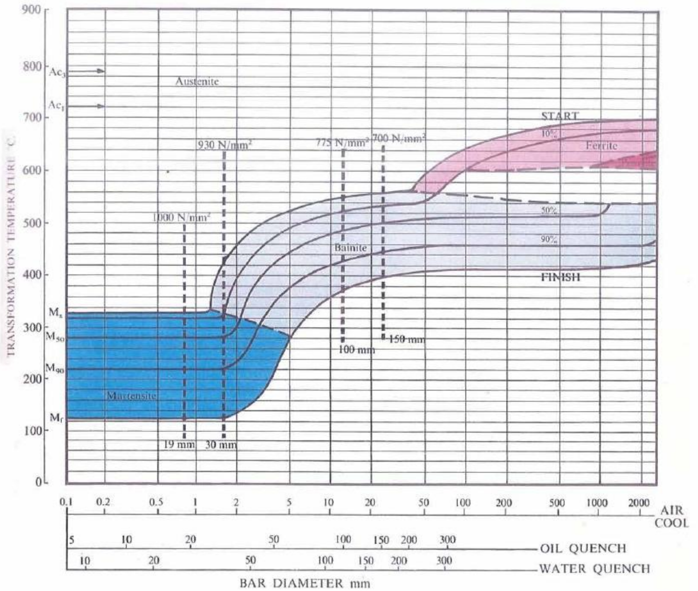
Fig 1/2 CCT diagram for 1 1/2 MnMo alloy steel (605M36) chosen to illustrate the microstructures to be expected after oil quenching at the various limiting ruling sections. Also indicated are the tensile strength levels after hardening and tempering taken from BS 970 Part 2 1970 (Based on CCT Diagram No. 40).
